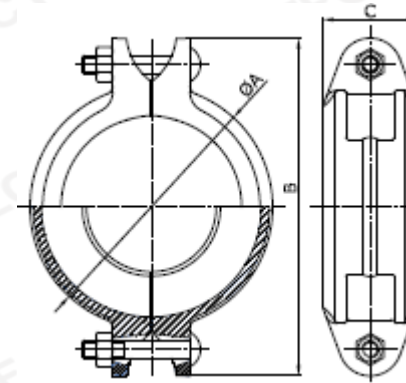
* Informational type cross section view. It does not represent a specific version on the Joint.
