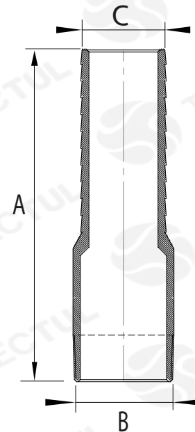
* Informational cross-sectional view. Does not represent a specific version of the accessory or item.
