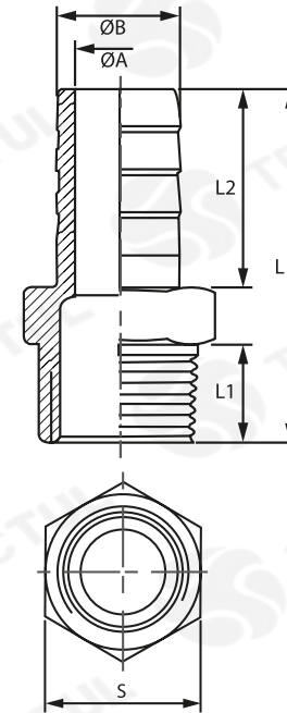
Informational type cross section view. It does not represent the specific version of the accessory.
